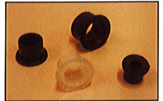
Plain Shouldered Nylon Bush Product Size and Code # 1/2" NB5 # 1750 12mm NB6 # 1751 3/8" NB3 # 1752 10mm NB4 # 1753 6mm NB2 # 1754
