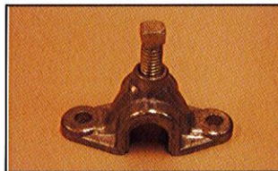
Blade Saddles - Full Circle Product Size and Code # 1/2" # 1761 12mm # 1763 3/8" # 1765 10mm # 1767
