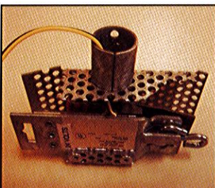
McCabe Electric Reuseable Bi-Metallic Thermal Link Temp Rated - 73 Deg. C (165 Deg. F) UL33 Tested - Complies AS1682.1 Product Code # 5721
