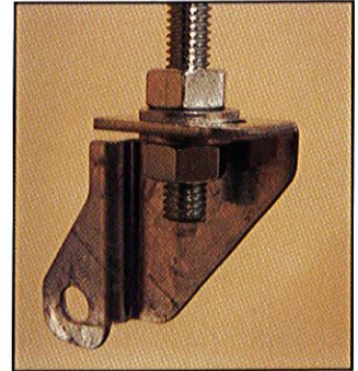
Bullock Ultimate Duct Hanger
