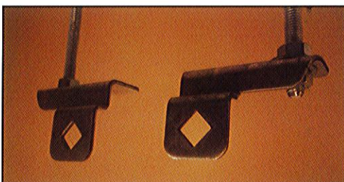
Bullock 35mm x 10ga Galvanised Duct Hangers
