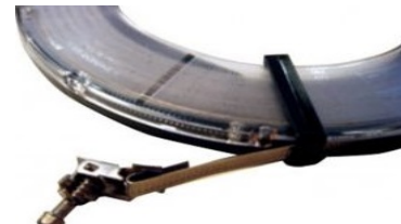
Stainless Steel Flexible Duct Banding 30m x 9mm Roll within plastic dispenser Code #1115
