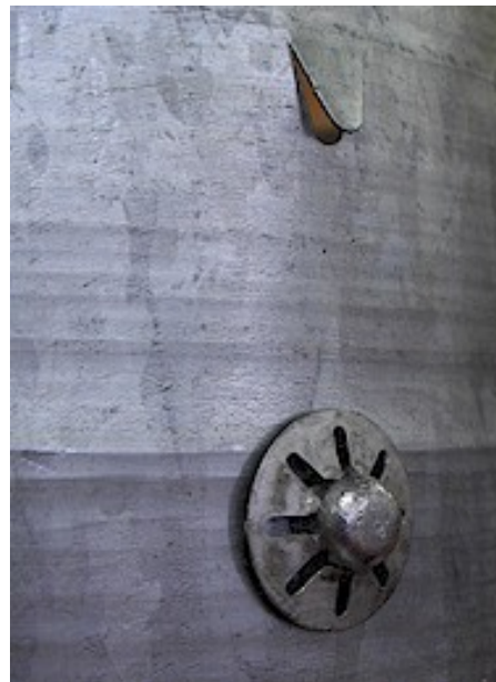
Blade bearing retaining clip and lance.
